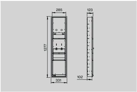
Item no.: 14710008012 Description: Sanitary Panel, Module size 8, Model HDK
