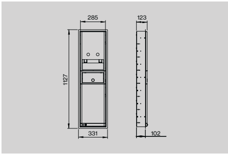
Item no.: 14710007073 Description: Sanitary Panel, Module size 7, Model HY
