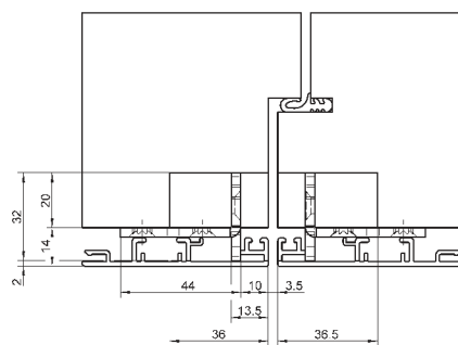
timber/aluminium system
