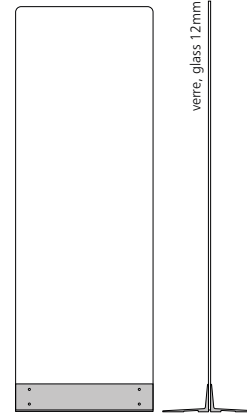
ile 224 S w 750 x h 2200 x d 512mm w 29,52 x h 86,61 x d 20,15"
